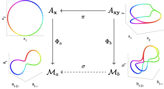
Fig. 3. Visual explanation of the cross map. We consider a two dimensional state \mathbf{x} \in \mathbb{R}^2 with an attractor A_x . We then suppose that \mathbf{x} causes \mathbf{y} \in \mathbb{R}^1 , and the joint state (\mathbf{x}, \mathbf{y}) has an attractor A_{xy} . The signals a_t and b_t are functions of \mathbf{x}_t and \mathbf{y}_t , respectively. The projection \pi(\mathbf{x}, \mathbf{y}) = \mathbf{x} maps A_{xy} onto A_x . The mappings \Phi_a, \Phi_b are diffeomorphisms which exist by Takens' theorem. The colors of points on each attractor and shadow manifold correspond uniquely to points in A_x . Using the colors to map points in \mathcal{M}_b to points in \mathcal{M}_a describes the cross map \sigma between the two shadow manifolds. Since \Phi_b is invertible, we see that the cross map is defined by \sigma(\mathbf{m}) = \Phi_a(\pi(\Phi_b^{-1}(\mathbf{m}))) .
