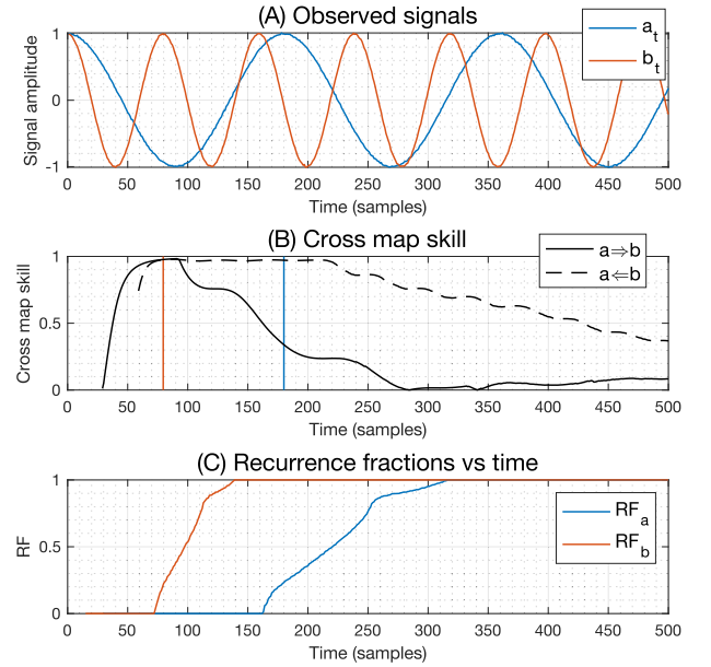
Fig. 7. Demonstration of the recurrence principle with a pair of sinusoids. (a) Two sine waves a_t and b_t signals are observed with frequencies f_a and f_b . The true causality is a \perp b . (b) The CCM convergence coefficient is observed against time. CCM asymptotically detects the true causality, but for a shorter time series (e.g., the first 200 samples), we would erroneously infer that a \Leftarrow b . The vertical lines mark one period of the sinusoids in (A). (c) The recurrence fraction RF as new data are received, for a particular choice of masking radii r_a and r_b . We observe that the convergence coefficients begin to decline shortly after when RF begins to increase.
