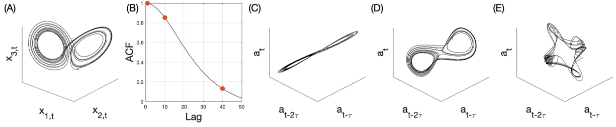
Fig. 2. Demonstration of SSR and the effect of the embedding delay parameter \tau . (a) An attractor in the Lorenz system [24]. The complete system state is latent, but we observe a signal a_t = x_{1,t} . (b) The autocorrelation function (ACF) of the signal a_t . The values of the ACF at 1, 10 and 40 are marked by the orange dots. (c) Shadow manifold \mathcal{M}_a produced by SSR when Q = 3 and \tau = 1 . Since the ACF at this \tau is close to 1, the coordinates of \mathbf{m}_t^a are highly correlated and \mathcal{M}_a is compressed to a line. (d) SSR result when Q = 3 and \tau = 10 . We see the shadow manifold appears to reconstruct the shape of the latent attractor in (A). (e) SSR result when Q = 3 and \tau = 40 . Although \mathcal{M}_a embeds the latent attractor, the embedding becomes more complicated as \tau increases. The ideal value of \tau for reconstructing the latent attractor lies between the extremes of (C) and (E) [18]. However, the shadow manifolds in (C-E) are equivalent to the original attractor in (A) up to nonlinear transformation.
