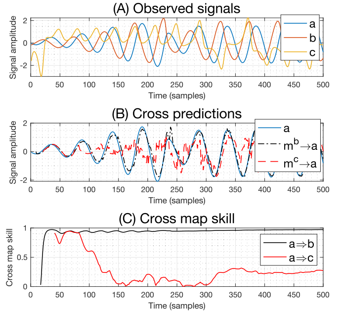
Fig. 4. Given a triplet of signals a_t, b_t, c_t , we use CCM to test a \Rightarrow b and a \Rightarrow c . (a) Observed signals. a_t, b_t, c_t are the x_1, x_2 and y_2 coordinates respectively of the Rössler-Lorenz system in (30), with zero coupling ( C = 0 ). (b) The signal a_t is estimated using \mathbf{m}_t^b to test a \Rightarrow b . Similarly, we estimate a_t from \mathbf{m}_t^c to test a \Rightarrow c . (c) For a \Rightarrow b , the cross map skill, \rho_t = \text{corr}(a_{1:t}, \hat{a}_{1:t}) , improves over time. Since the cross map skill converges to something near 1, we conclude that a_t causes b_t . In contrast, the asymptotic cross map skill for a \Rightarrow c is poor, so we conclude that a_t does not drive c_t . As t \rightarrow \infty , the cross map skill should tend to 0, but it may take some time for the cross map skill to decay sufficiently.
